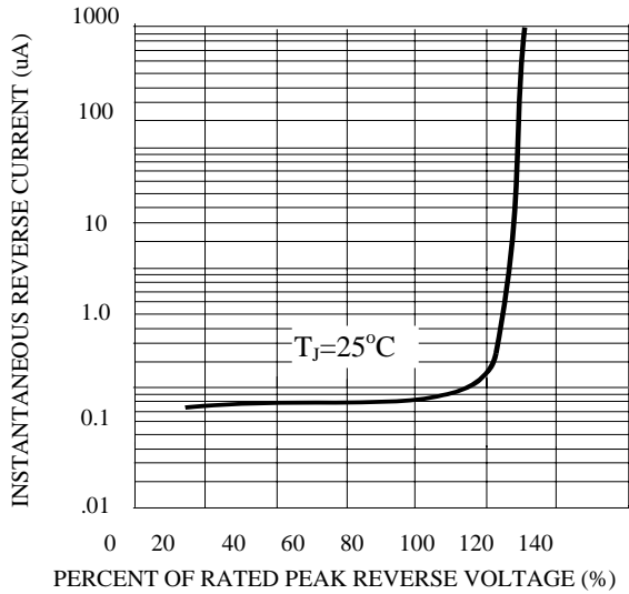
FIG. 3-TYPICAL REVERSE CHARACTERISTICS
